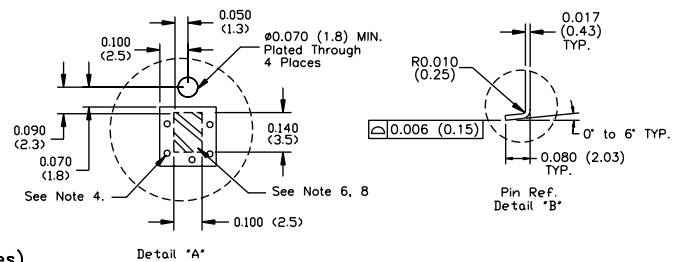
PC Layout
