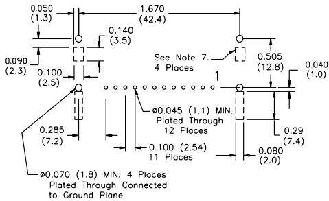
PC Layout
