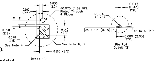
PC Layout
