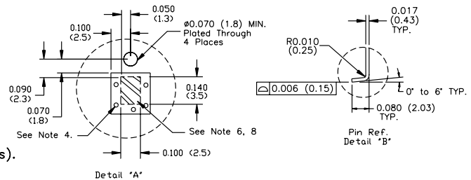
PC Layout
