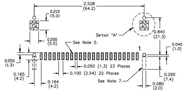
PC Layout
