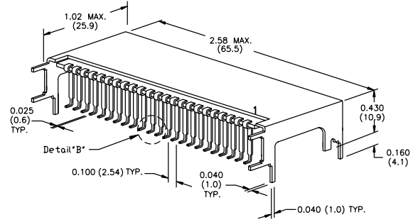
Horizontal Surface Mount (Suffix C)
