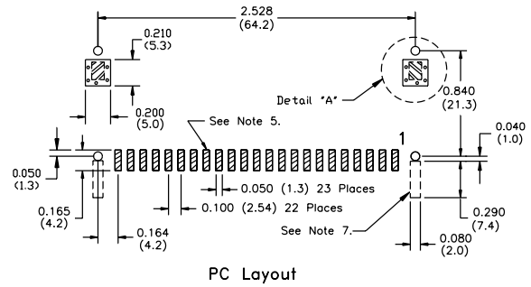
PC Layout
